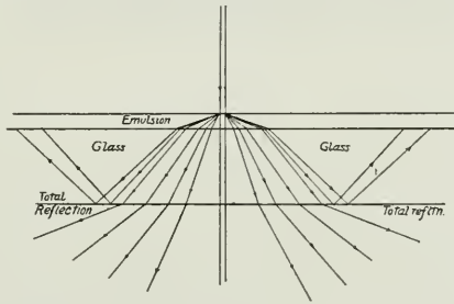
Fig. 97. Rays in Photographic Plate.
